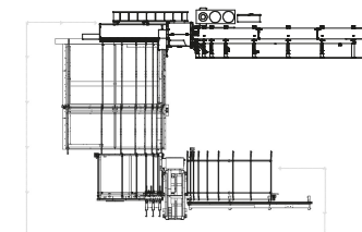
U-SFC LAYOUT
